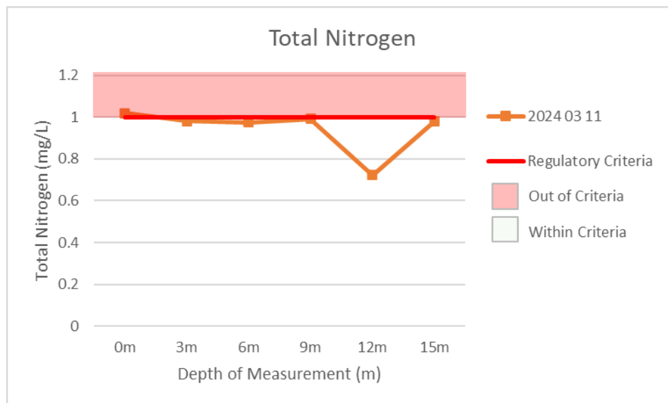
Figure 6: Total nitrogen from Kemmerer samples in West Basin of LLB Lake - 2024
