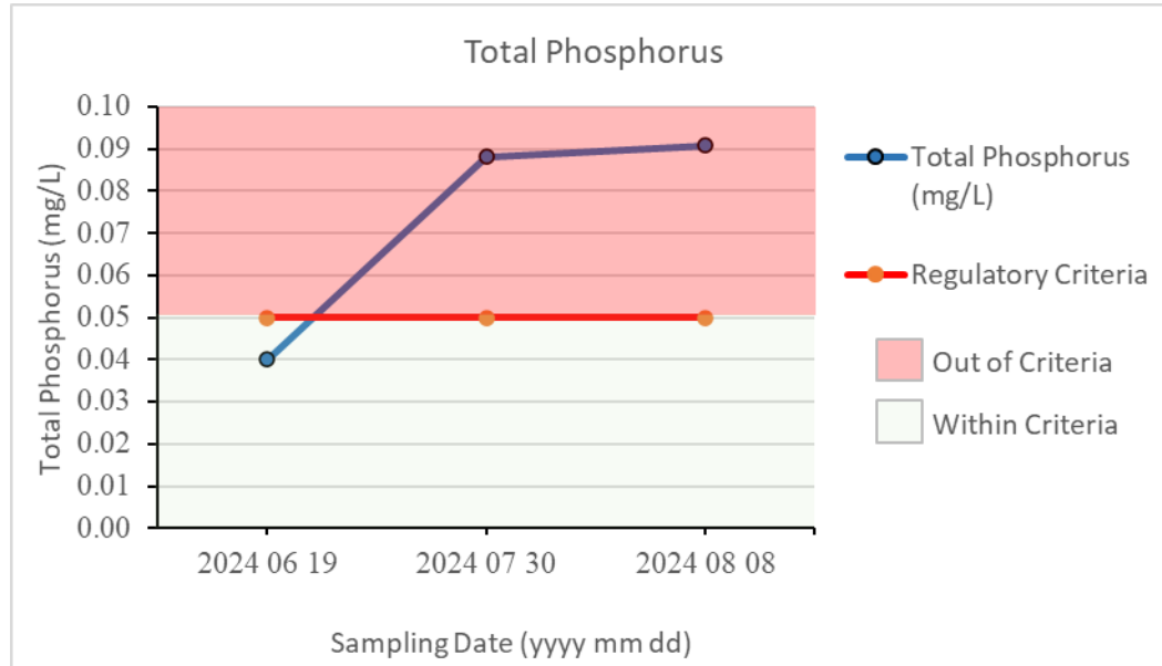
Figure 7: Total phosphorus from composite samples in West Basin of LLB Lake – 2024
