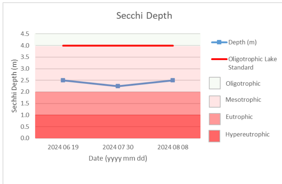
Figure 2: Secchi depths measured in West Basin of LLB Lake – 2024
