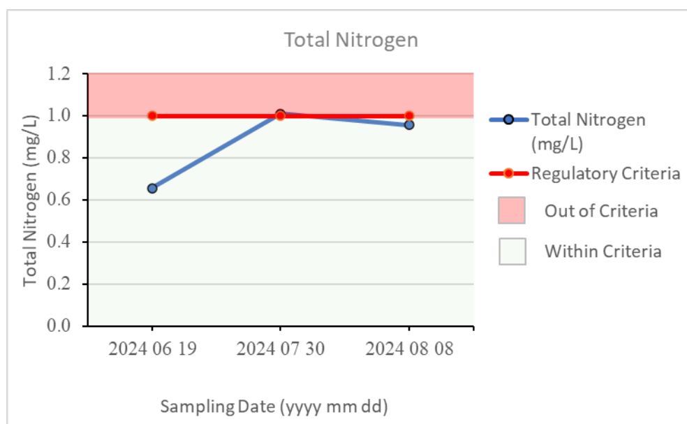
Figure 5: Total nitrogen from composite samples in West Basin of LLB Lake - 2024
