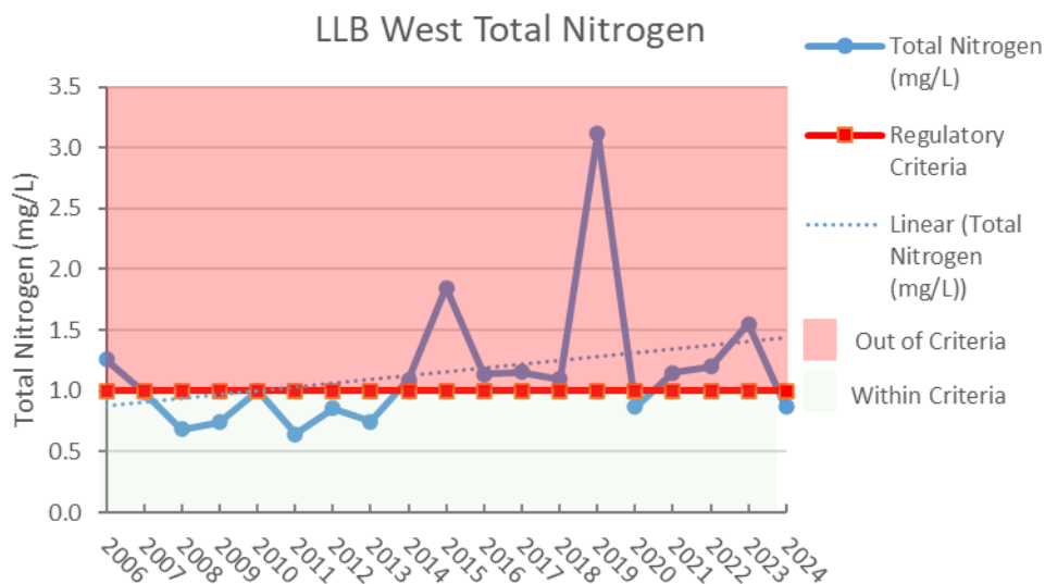
Figure 14: Historical trend of total nitrogen in West Basin of LLB Lake
