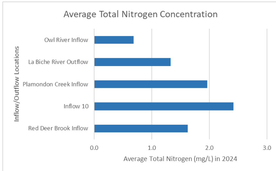
Figure 9: Inflow and outflow total nitrogen concentration for Lac La Biche Lake – 2024
