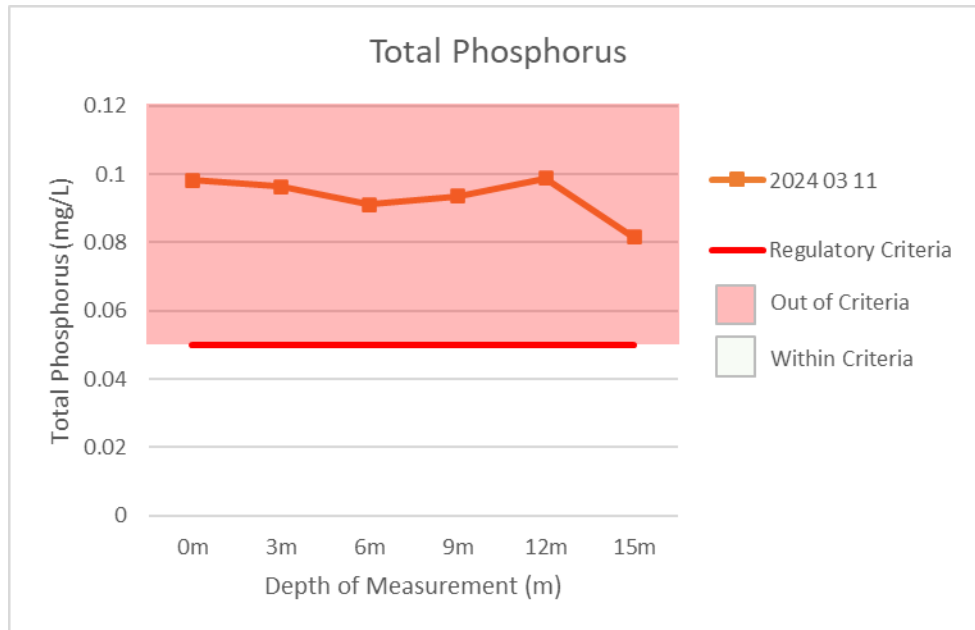
Figure 8: Total phosphorus from Kemmerer samples in West Basin of LLB Lake – 2024
