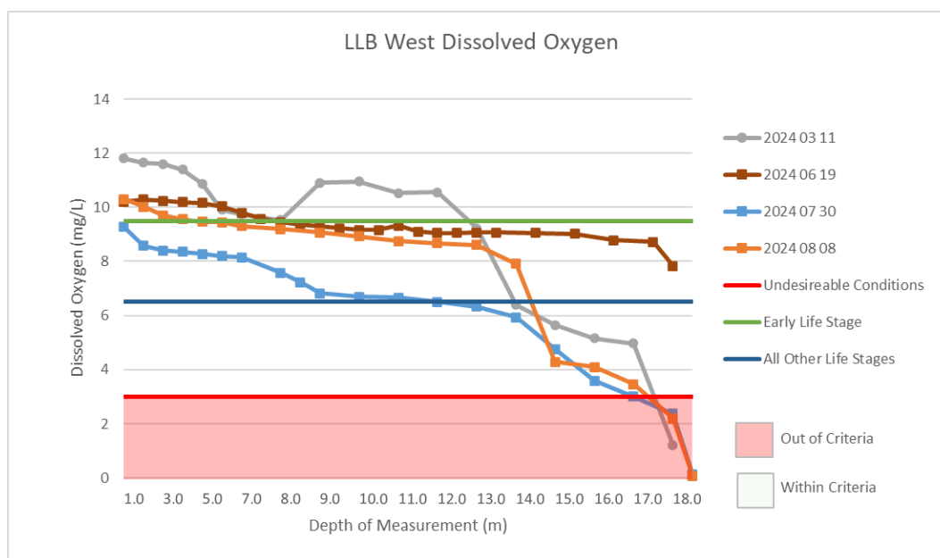
Figure 3: Dissolved oxygen in West Basin of LLB Lake - 2024
