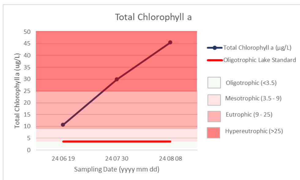
Figure 11: Total Chlorophyll-a from Composite samples of the West Basin in LLB Lake - 2024
