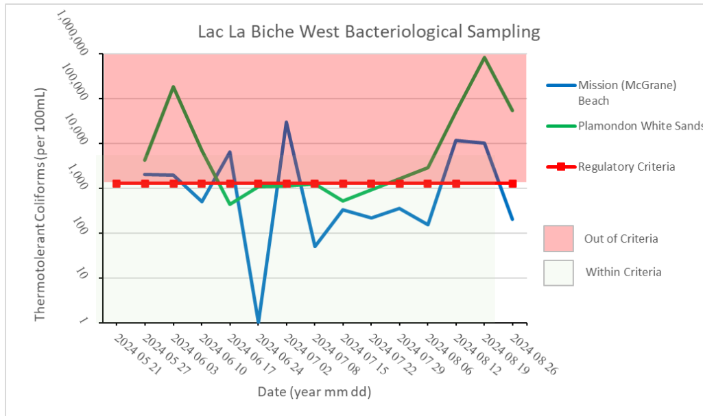
Figure 12: Enterococcus counts from McArthur Beach – 2024
