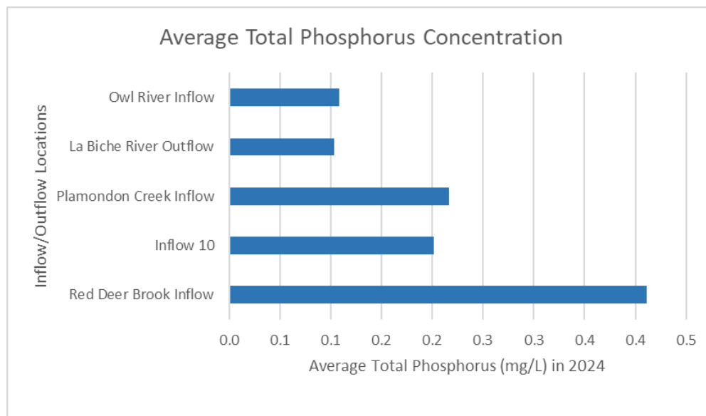
Figure 10: Inflow and outflow total phosphorous concentration for Lac La Biche Lake – 2024
