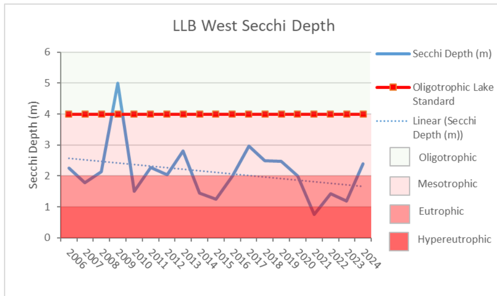
Figure 13: Historical trend of Secchi depth in West Basin of LLB Lake
