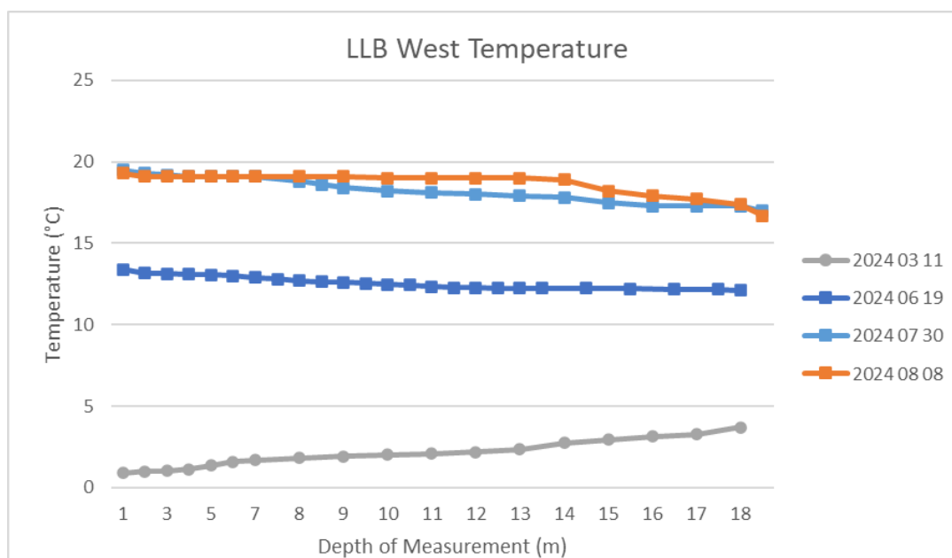
Figure 4: Temperature profile in West Basin of LLB Lake - 2024
