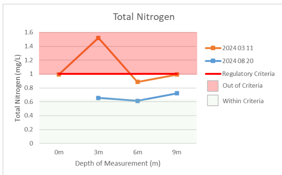
Figure 6: Total nitrogen from Kemmerer samples in East Basin of LLB Lake - 2024
