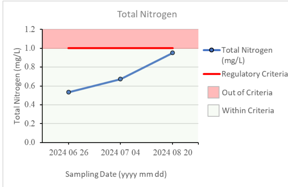
Figure 5: Total nitrogen from composite samples in East Basin of LLB Lake – 2024
