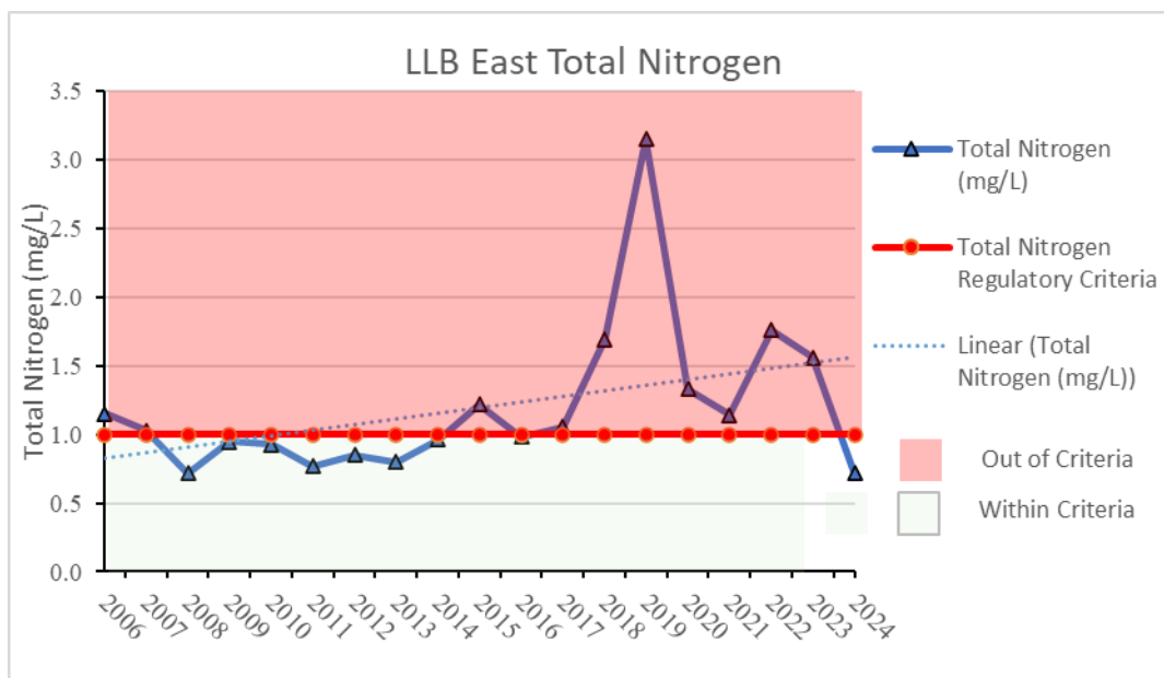
Figure 14: Historical trend of total nitrogen in East Basin of Lac La Biche Lake
