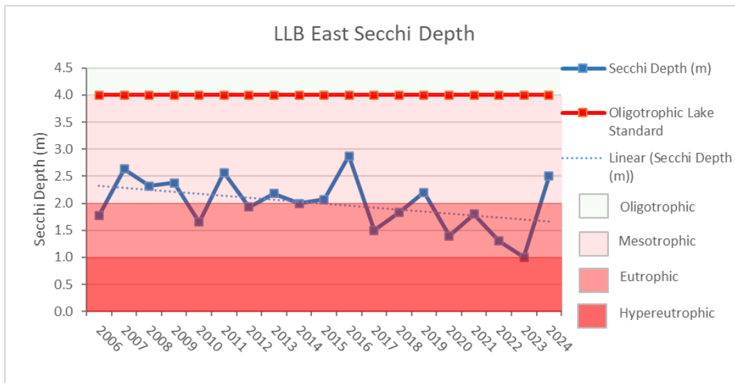
Figure 13: Historical trend for Secchi Depth in East Basin of Lac La Biche Lake
