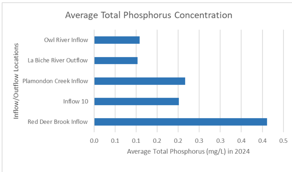
Figure 10: Inflow and outflow total phosphorus concentration for Lac La Biche Lake – 2024
