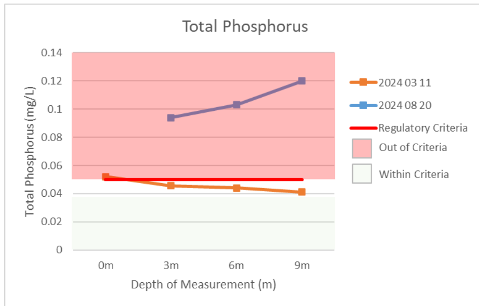
Figure 8: Total phosphorus from Kemmerer samples in East Basin of LLB Lake - 2024
