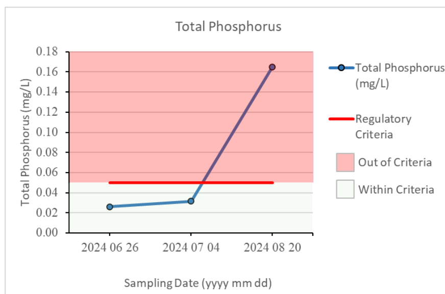
Figure 7: Total phosphorus from composite samples in East Basin of LLB Lake – 2024
