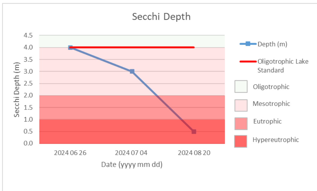
Figure 2: Secchi depths measured in East Basin of Lac La Biche Lake – 2024
