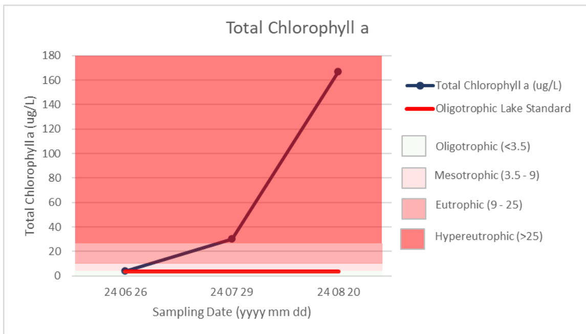
Figure 11: Total Chlorophyll-a from Composite samples in East Basin of LLB Lake - 2024
