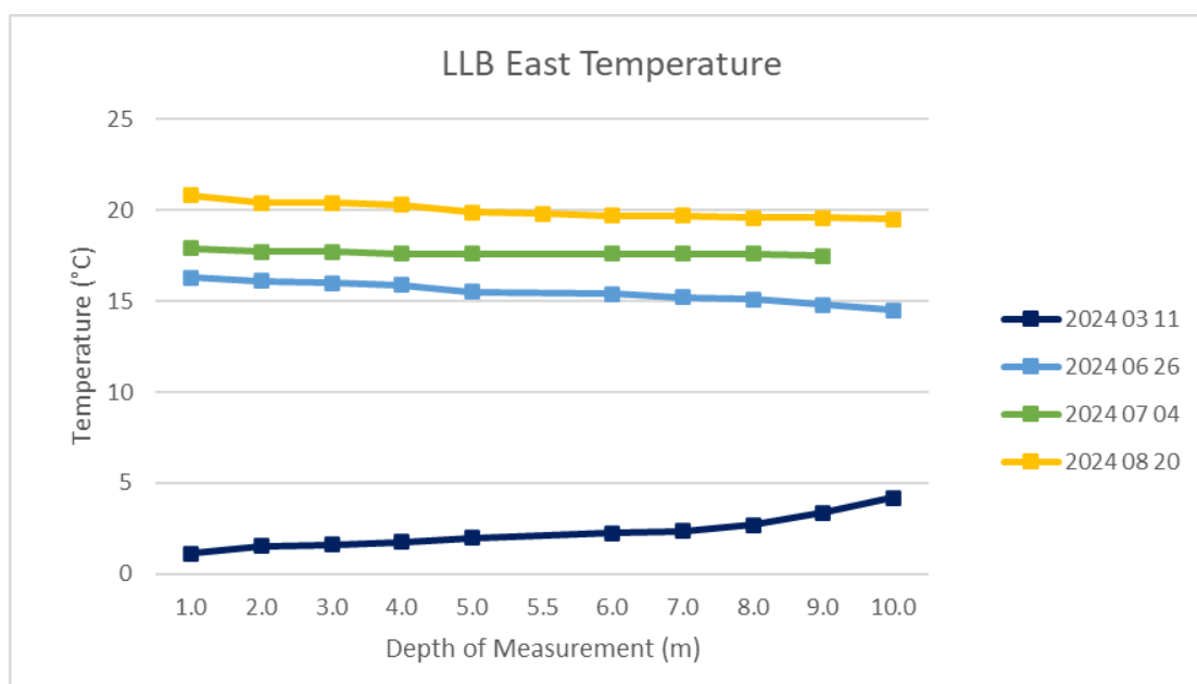
Figure 4: Temperature profile for East Basin of Lac La Biche Lake – 2024
