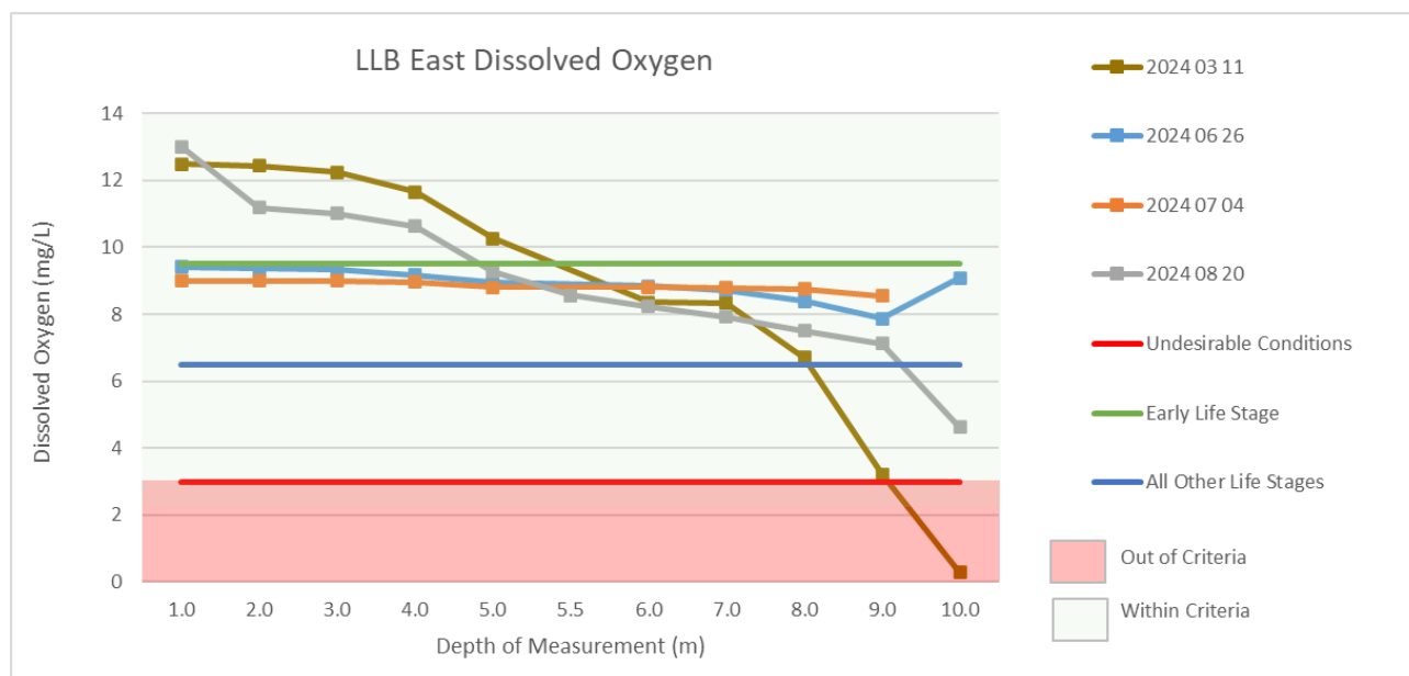
Figure 3: Dissolved oxygen in East Basin of Lac La Biche Lake – 2024
