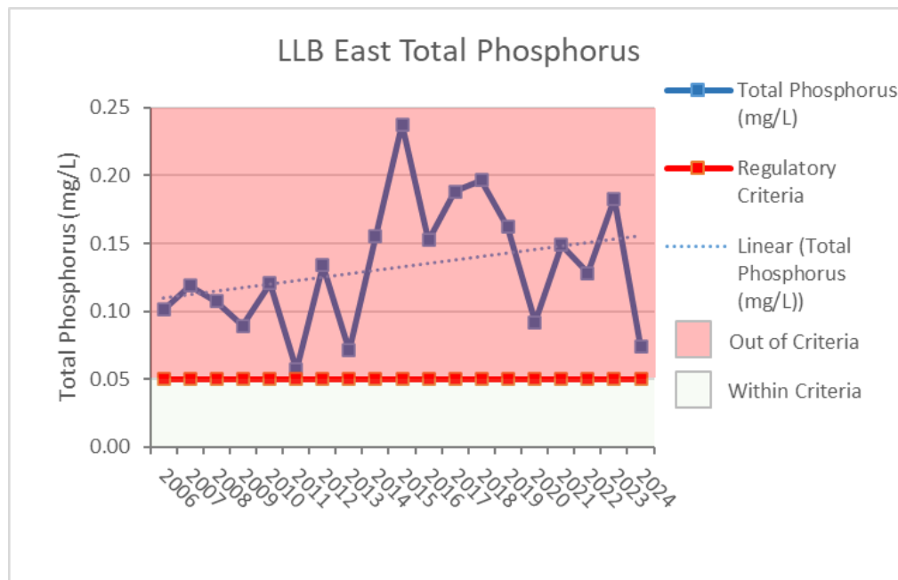
Figure 15: Historical trend of total phosphorus in East Basin of Lac La Biche Lake
