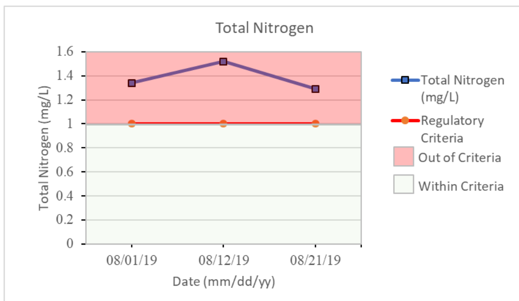
Figure 5: Total nitrogen from composite samples of Elinor Lake – 2019
