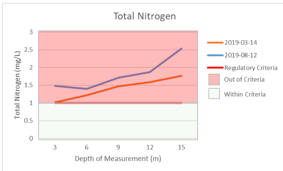
Figure 6: Total nitrogen from Kemmerer samples of Elinor Lake – 2019
