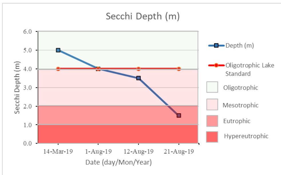
Figure 2: Secchi depth measurements in Elinor Lake - 2019
