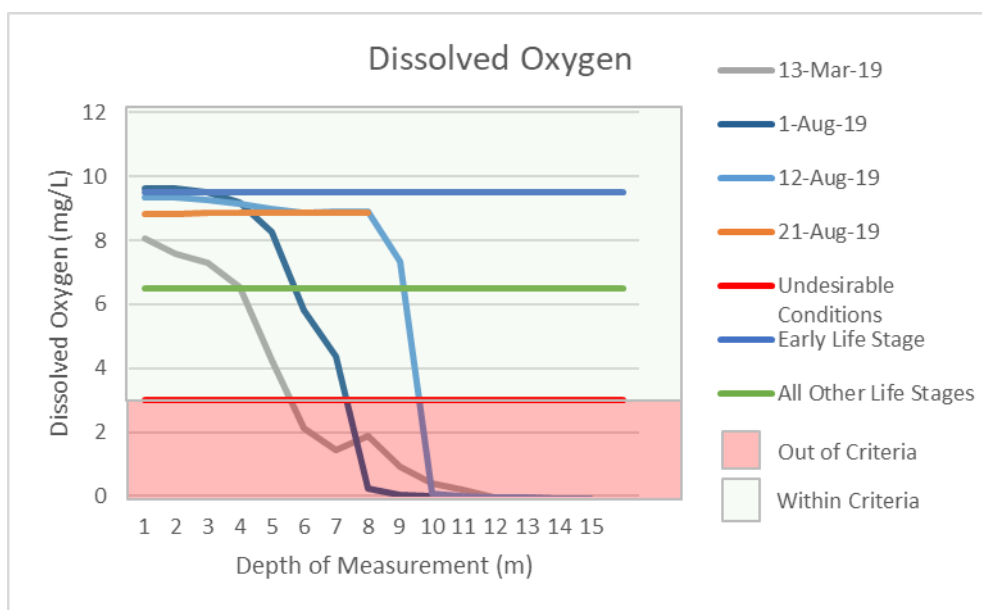
Figure 3: Dissolved oxygen in in Elinor Lake – 2019
