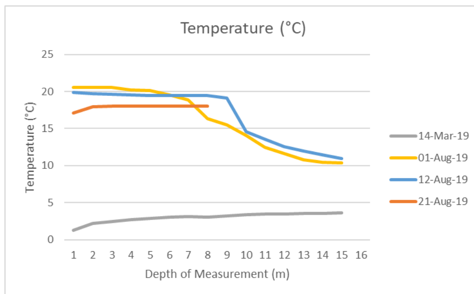
Figure 4: Elinor Lake temporal and spatial temperature measurements – 2019
