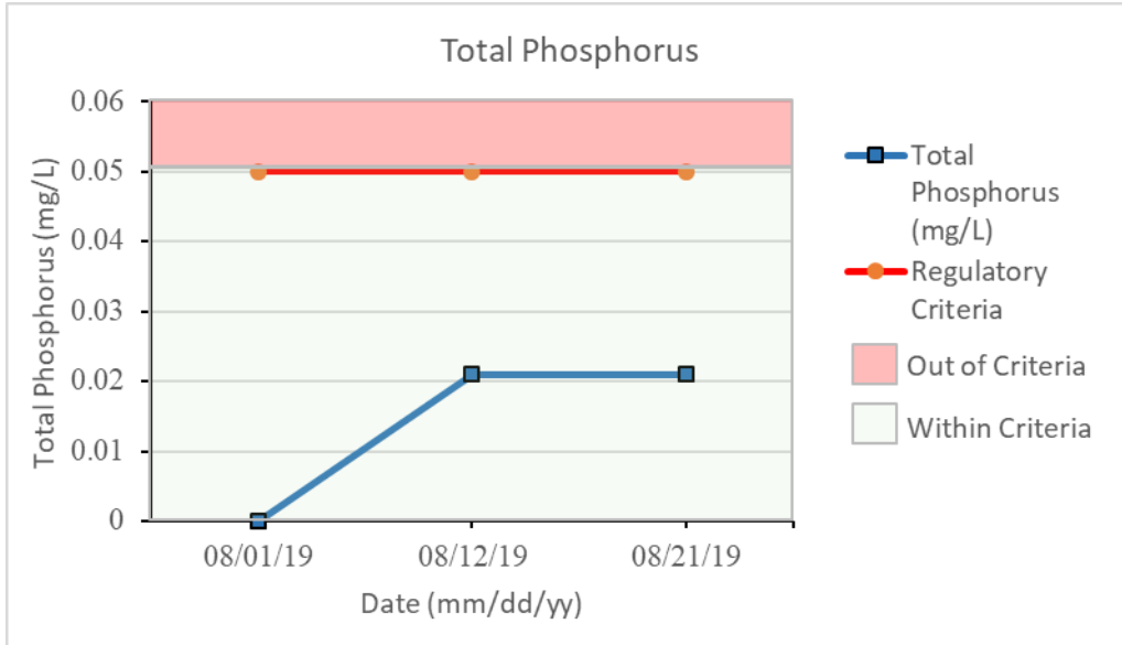
Figure 7: Total phosphorus from composite samples of Elinor Lake - 2019
