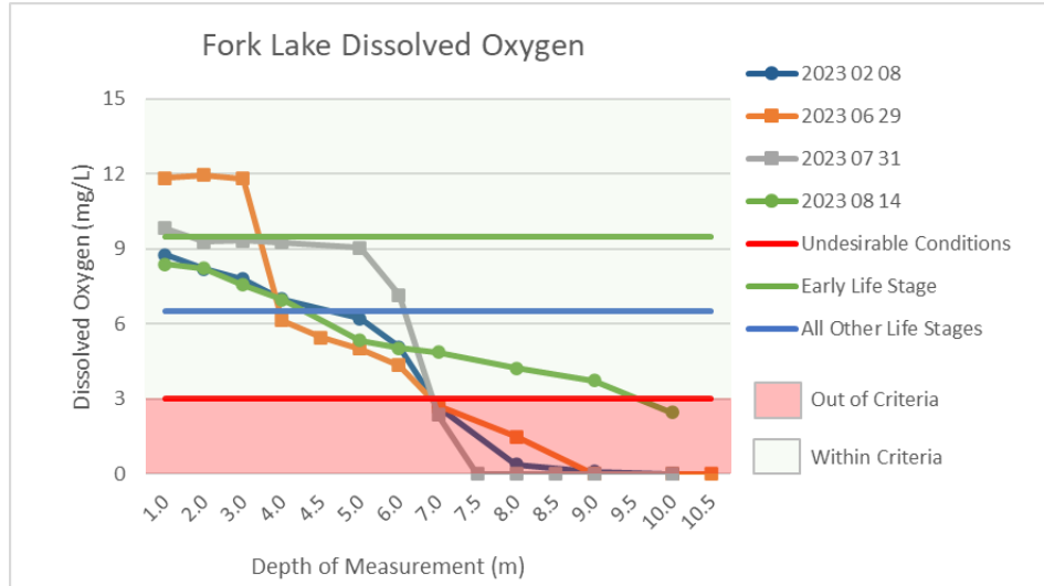
Figure 3: Dissolved oxygen in Fork Lake – 2023
