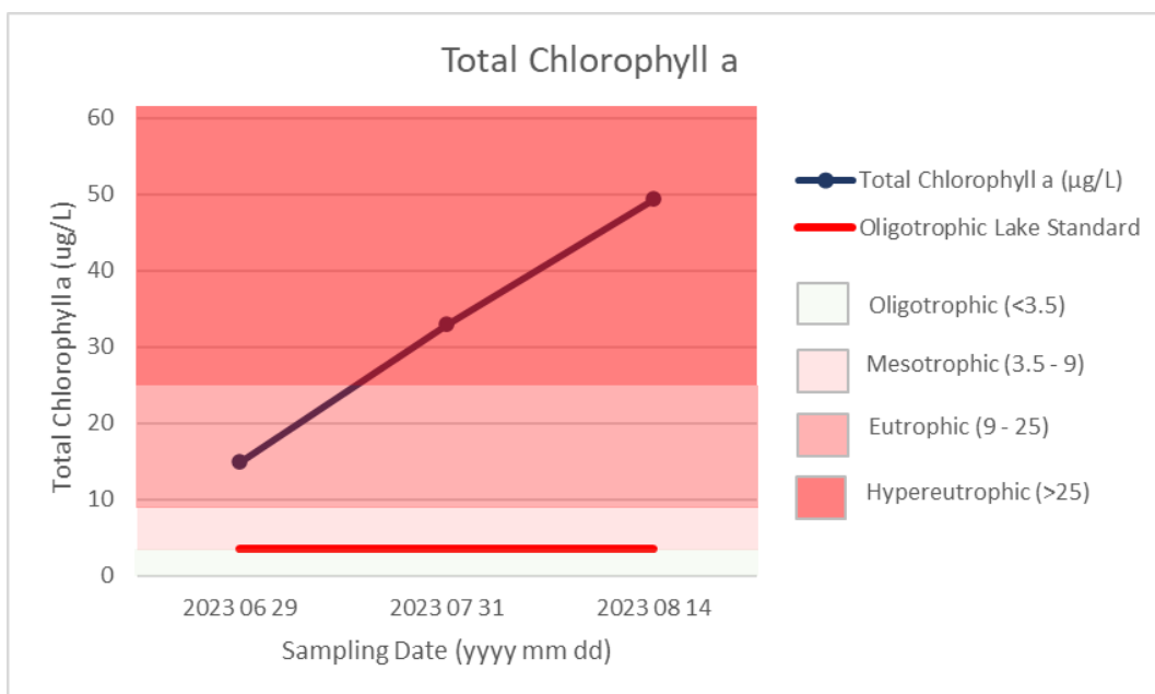
Figure 9: Total Chlorophyll-a in Composite samples of Fork Lake - 2023
