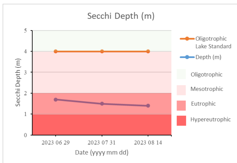
Figure 2: Secchi depths measured in Fork Lake – 2023
