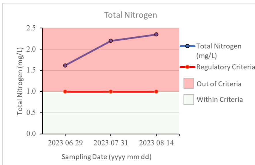
Figure 5: Total nitrogen from composite samples of Fork Lake – 2023
