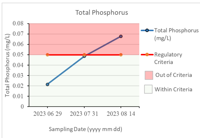
Figure 7: Total phosphorus in composite samples of Fork Lake - 2023
