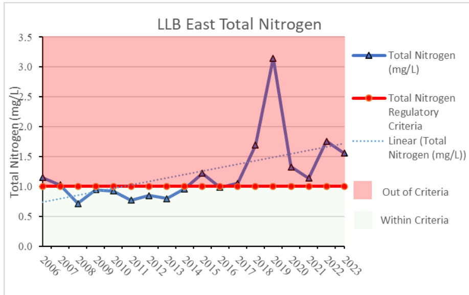
Figure 14: Historical trend of total nitrogen in East Basin of Lac La Biche Lake
