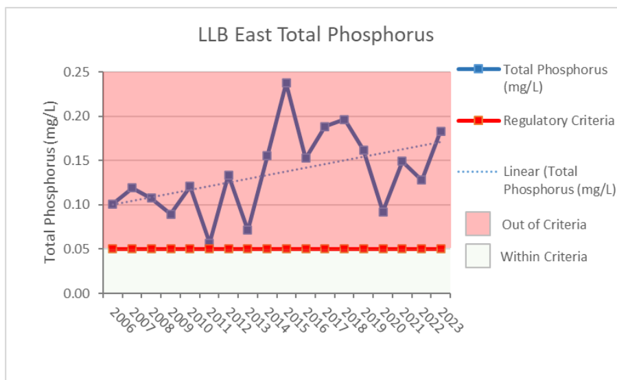
Figure 15: Historical trend of total phosphorus in East Basin of Lac La Biche Lake
