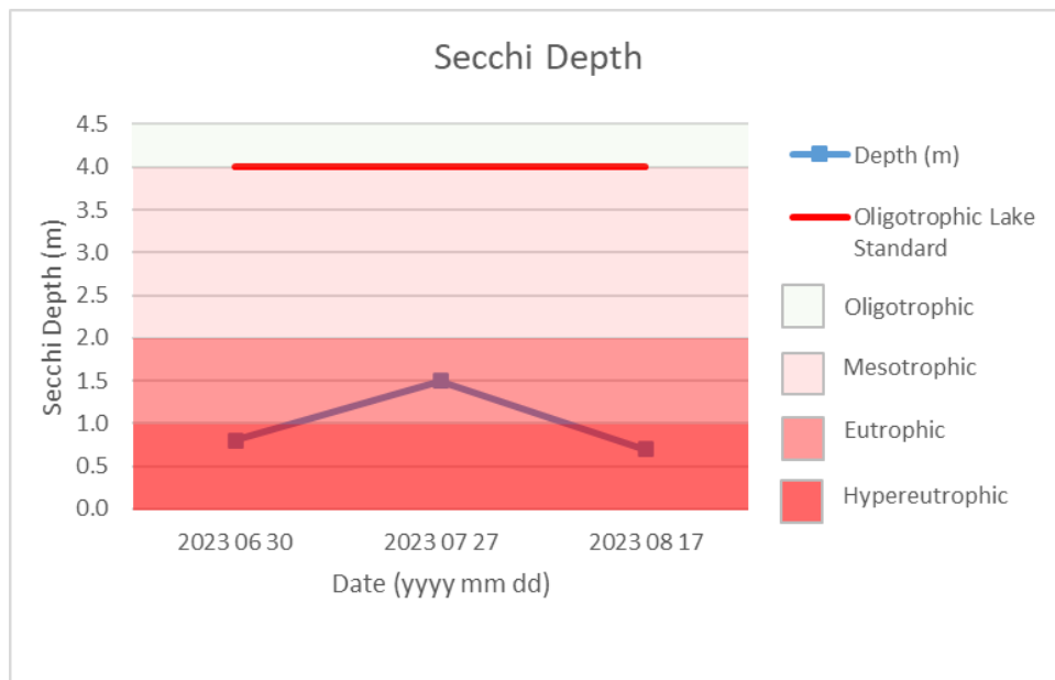
Figure 2: Secchi depths measured in East Basin of Lac La Biche Lake – 2023
