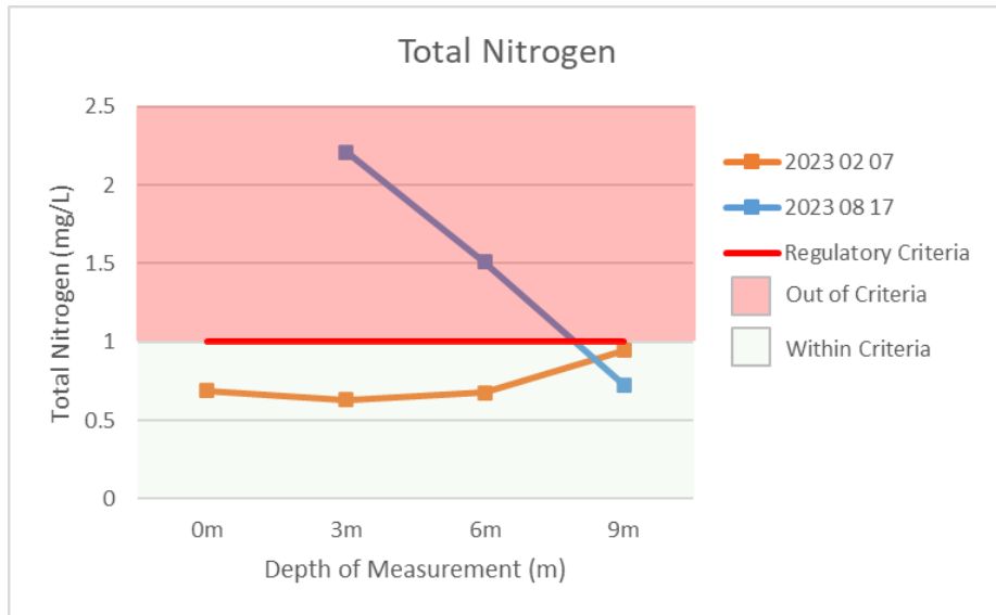
Figure 6: Total nitrogen from Kemmerer samples in East Basin of LLB Lake - 2023
