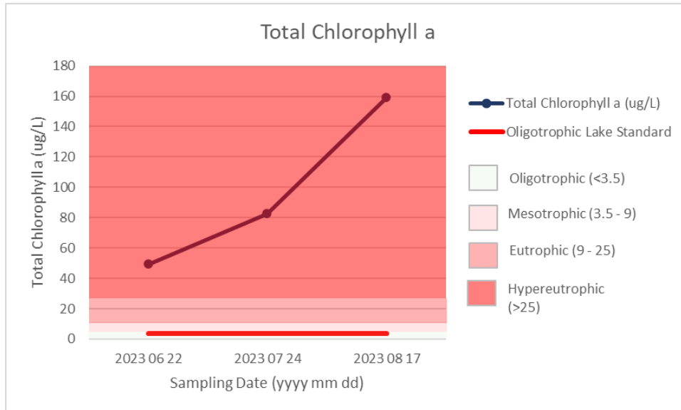
Figure 11: Total Chlorophyll-a from Composite samples in East Basin of LLB Lake - 2023
