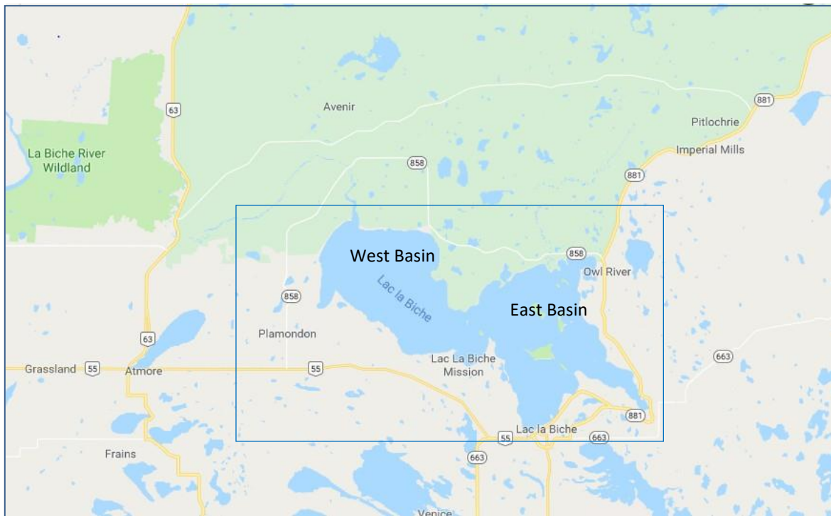
Figure 1: Location map of Lac La Biche Lake
