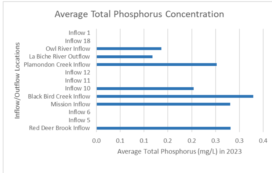
Figure 10: Inflow and outflow total phosphorus concentration for Lac La Biche Lake – 2023
