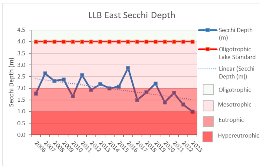
Figure 13: Historical trend for Secchi Depth in East Basin of Lac La Biche Lake
