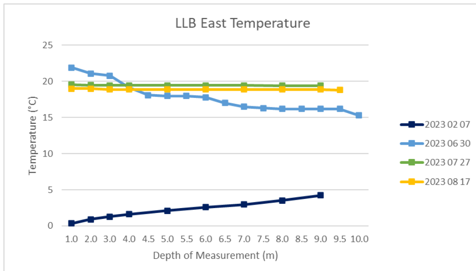
Figure 4: Temperature profile for East Basin of Lac La Biche Lake – 2023
