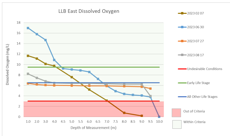
Figure 3: Dissolved oxygen in East Basin of Lac La Biche Lake – 2023
