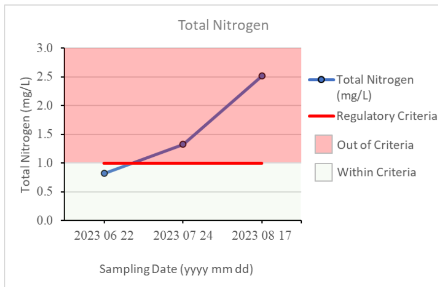
Figure 5: Total nitrogen from composite samples in East Basin of LLB Lake – 2023
