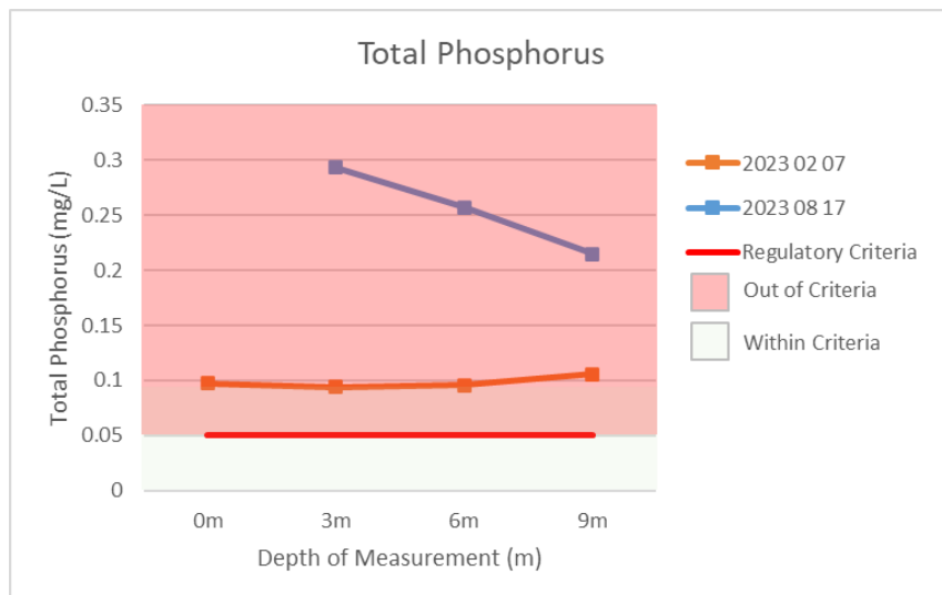
Figure 8: Total phosphorus from Kemmerer samples in East Basin of LLB Lake - 2023
