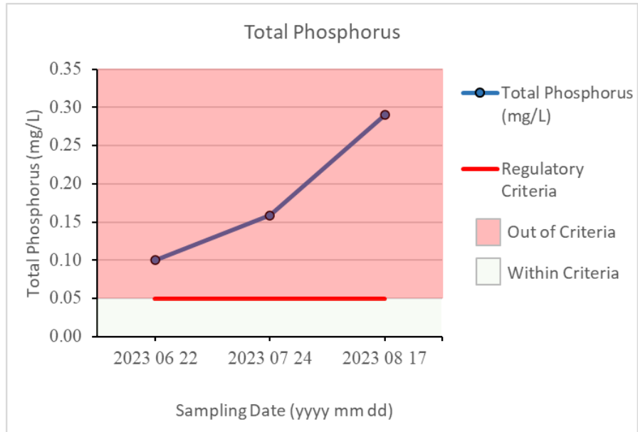
Figure 7: Total phosphorus from composite samples in East Basin of LLB Lake – 2023
